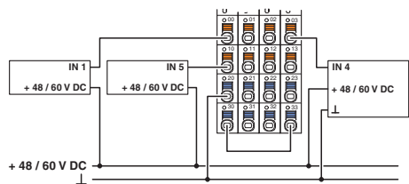
Connection of sensors when using external busbars
